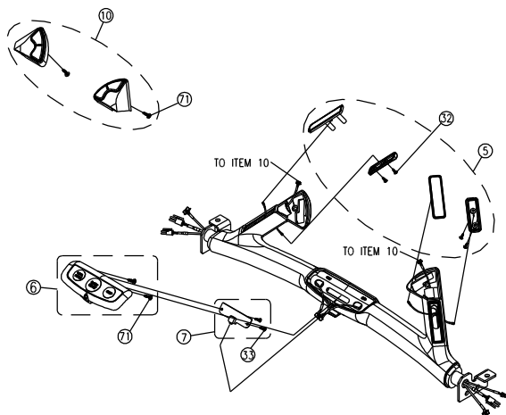
DETAIL VIEW OF CROSSBAR
