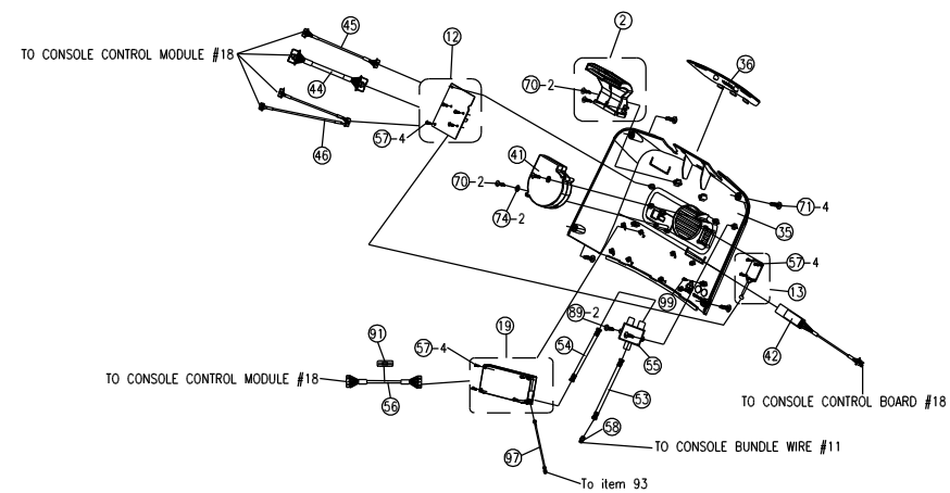
DETAIL VIEW OF BACK COVER
